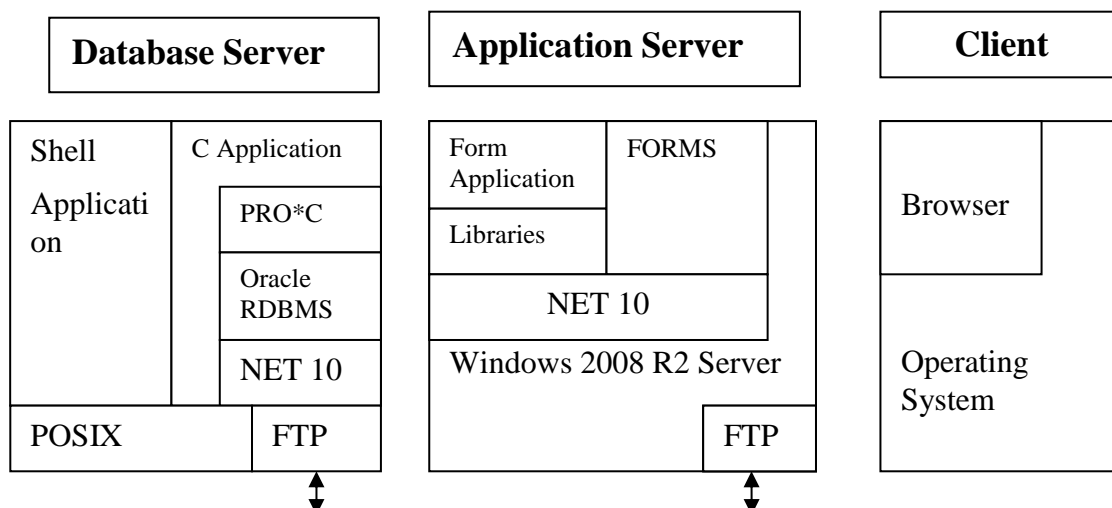
Figure 11: ISRA Software Architecture
