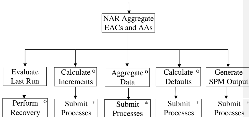
Figure 5: NAR Aggregate EACs and AAs
