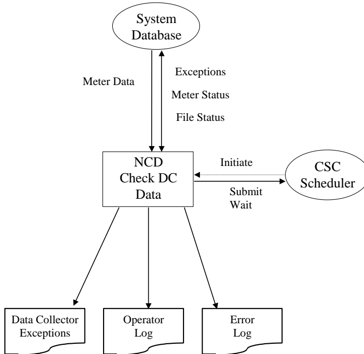
Figure 6: Context Diagram for Check DC Data
