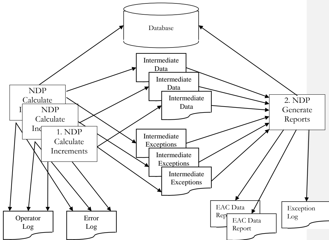
Figure 11: NDP Processing Flow
