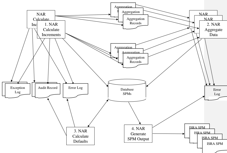
Figure 4: NAR Processing Flow
