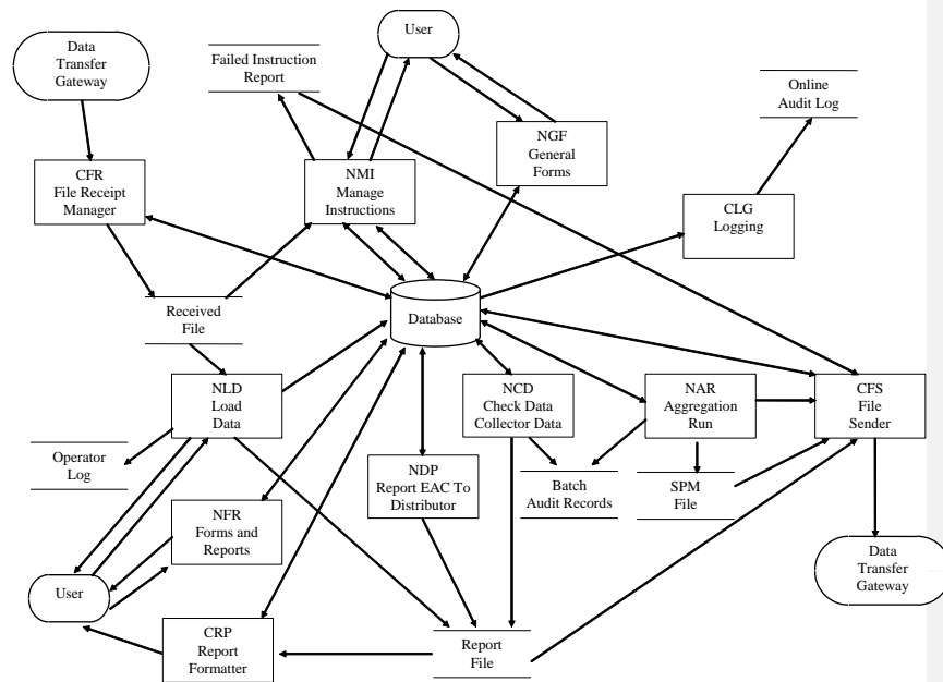
Figure 1: NHHDA System Overview
