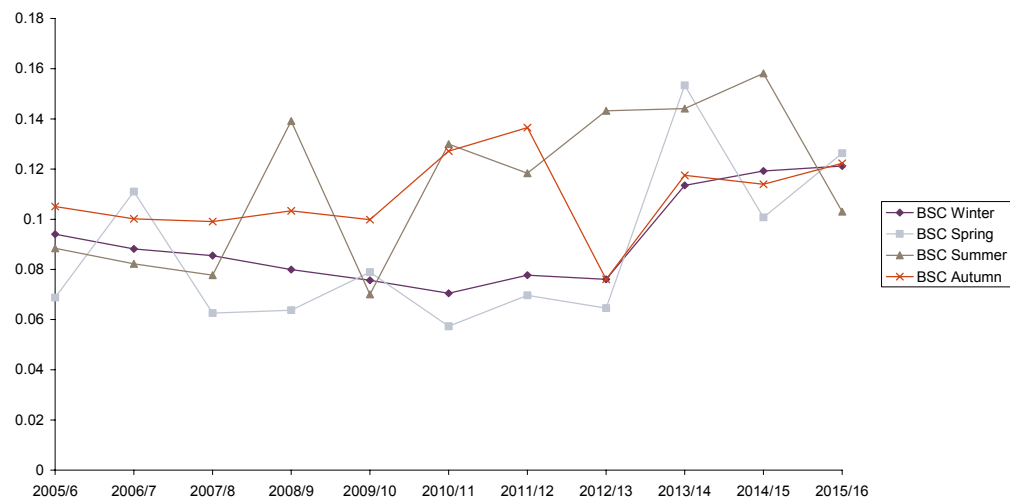
Figure 3.10 Seasonal betas
